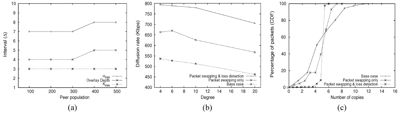
Fig. 9. (a) K_{min} , depth and \omega_{min} for different peer populations. (b) Diffusion rate to level 1 across various peer degrees in three scenarios: source without any coordination, source with only packet swapping and source with both packet swapping and loss detection. (c) Distribution of the number of copies of each packet that are delivered to level 1 for peer degree 10 in the three scenarios.
