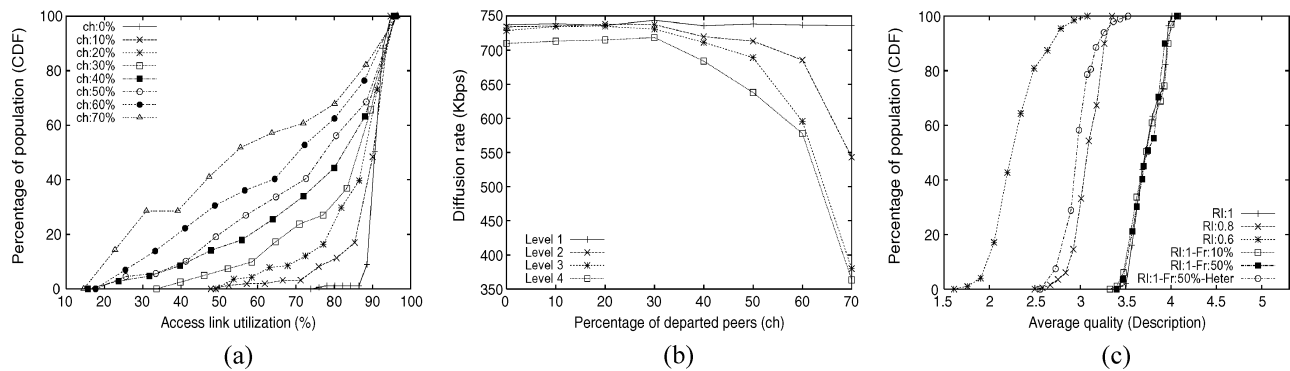
Fig. 11. (a) Distribution of utilization of access link bandwidth among peers for various percentages of ch . (b) Diffusion rate to different levels for various percentages of ch . (c) Distribution of average delivered quality (layers) to each peer for various RIs and for scenarios with different percentage of free-riders with RI = 1 . The result for 50% free-riders in a heterogeneous scenario is also included (RI:1-Fr:50%-Heter).
