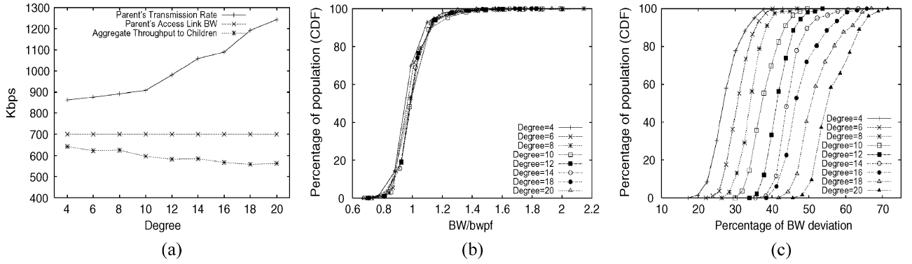
Fig. 5. (a) Transmission rate of a selected peer along with its access link bandwidth and aggregate throughput to all of its children. (b) Distribution of BW/bw_{pf} values across all connections. (c) Distribution of the deviation of aggregate bandwidth across all peers.
