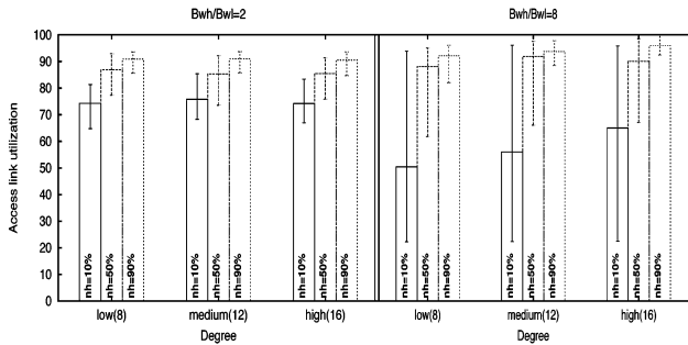
Fig. 1. Utilization of access link bandwidth across different peer degree and various level of heterogeneity, when all peers have the same incoming and outgoing degree regardless of their bandwidth.
